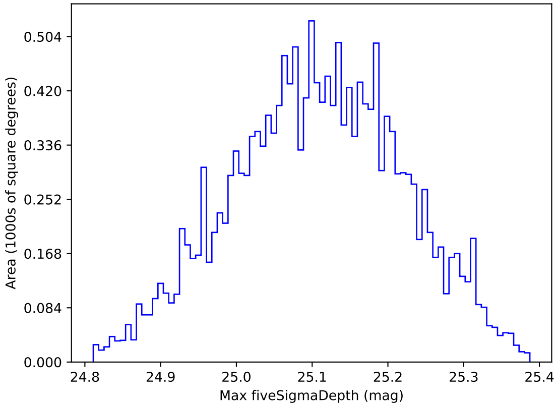
ddf_acor_sf10_lsf20_lsr10_v3.4_10yrs WFD g band: Max fiveSigmaDepth
