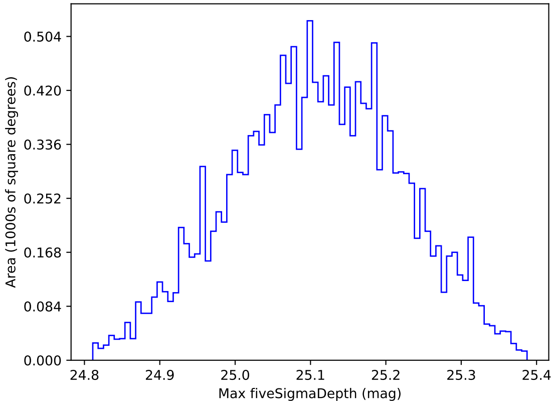
ddf_acor_sf10_lsf20_lsr10_v3.4_10yrs WFD all bands: Max fiveSigmaDepth
