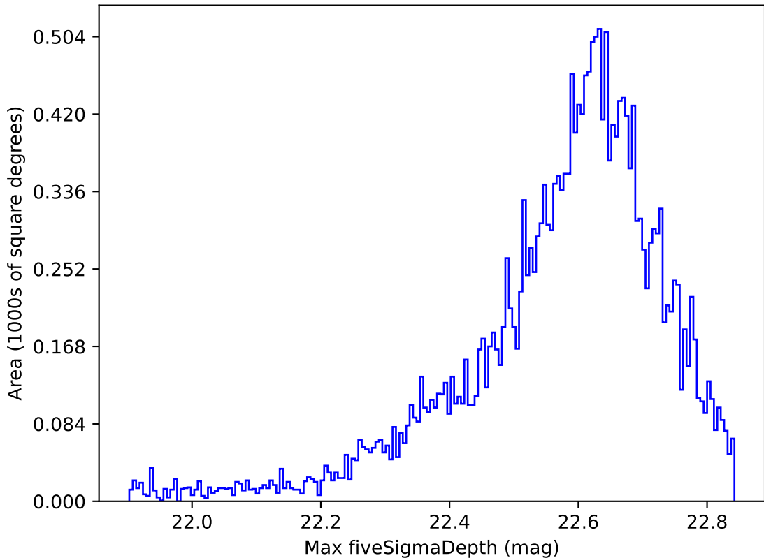
ddf_acor_sf10_ls20_lsr10_v3.4_10yrs All sky y band: Max fiveSigmaDepth
