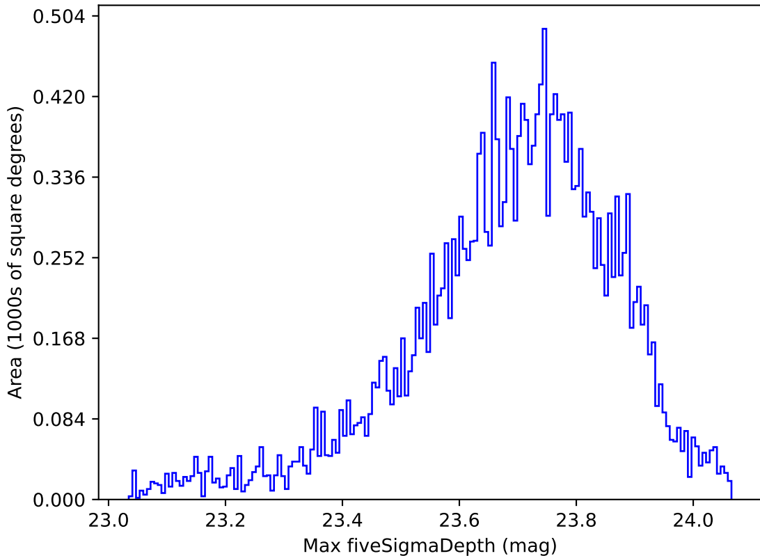
ddf_acor_sf10_ls20_lsr10_v3.4_10yrs All sky u band: Max fiveSigmaDepth
