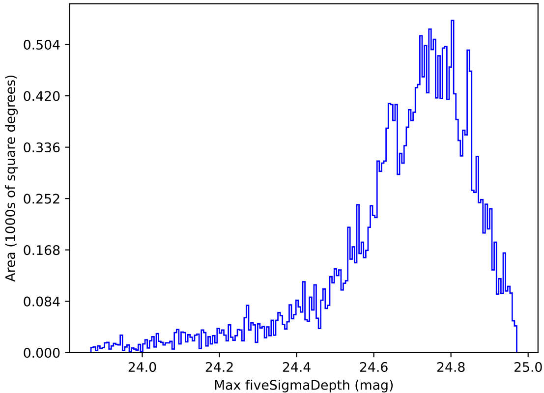
ddf_acor_sf10_lsf20_lsr10_v3.4_10yrs All sky r band: Max fiveSigmaDepth
