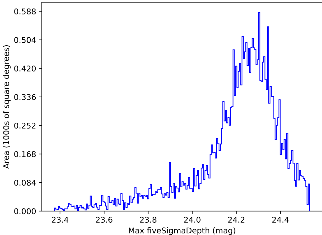
ddf_acor_sf10_lsf20_lsr10_v3.4_10yrs All sky i band: Max fiveSigmaDepth
