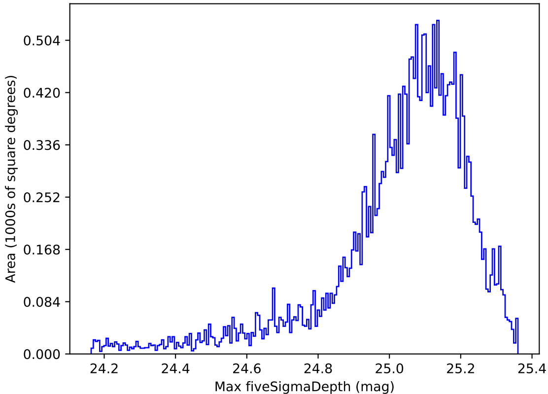
ddf_acor_sf10_ls20_lsr10_v3.4_10yrs All sky g band: Max fiveSigmaDepth
