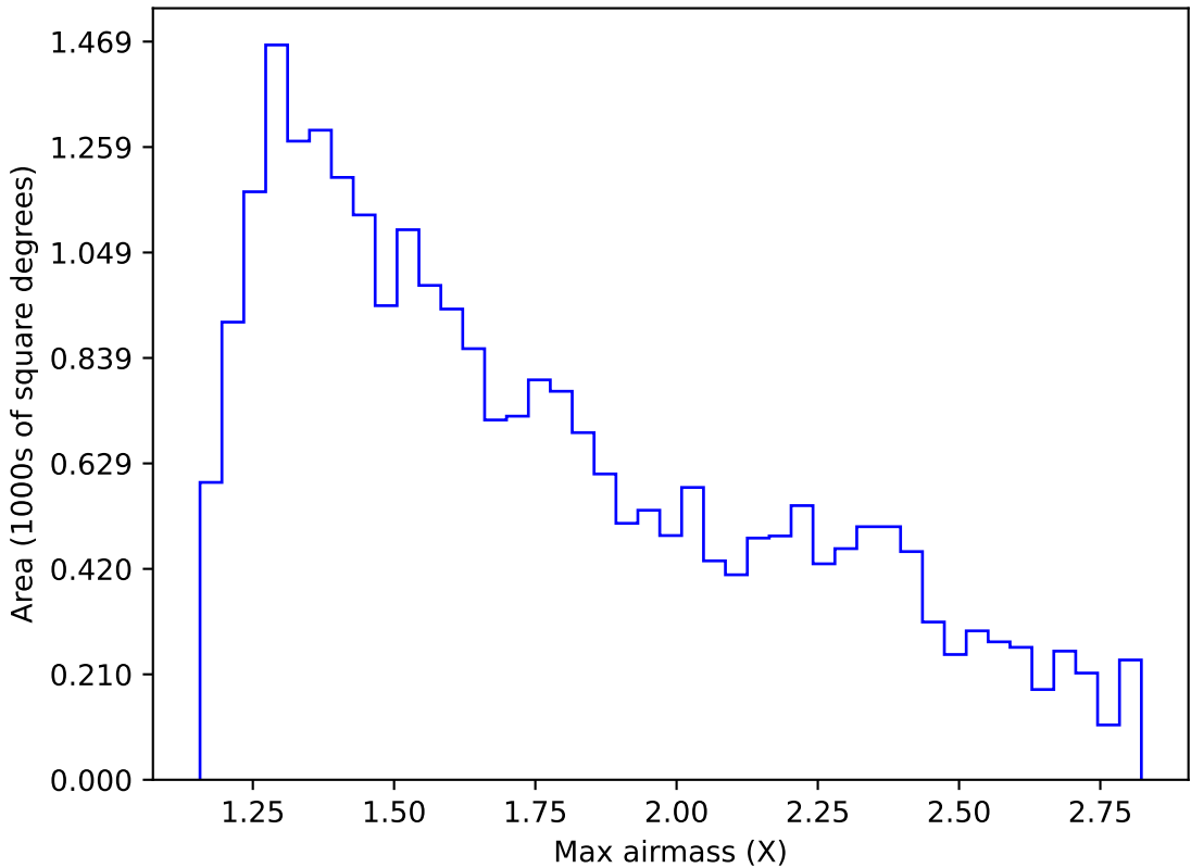
ddf_acor_sf10_lsf20_lsr10_v3.4_10yrs Yr 1 z band: Max airmass
