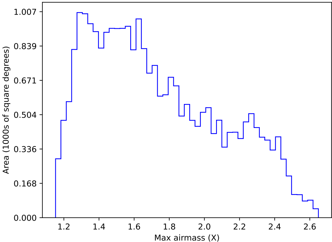
ddf_acor_sf10_lsf20_lsr10_v3.4_10yrs Yr 1 r band: Max airmass
