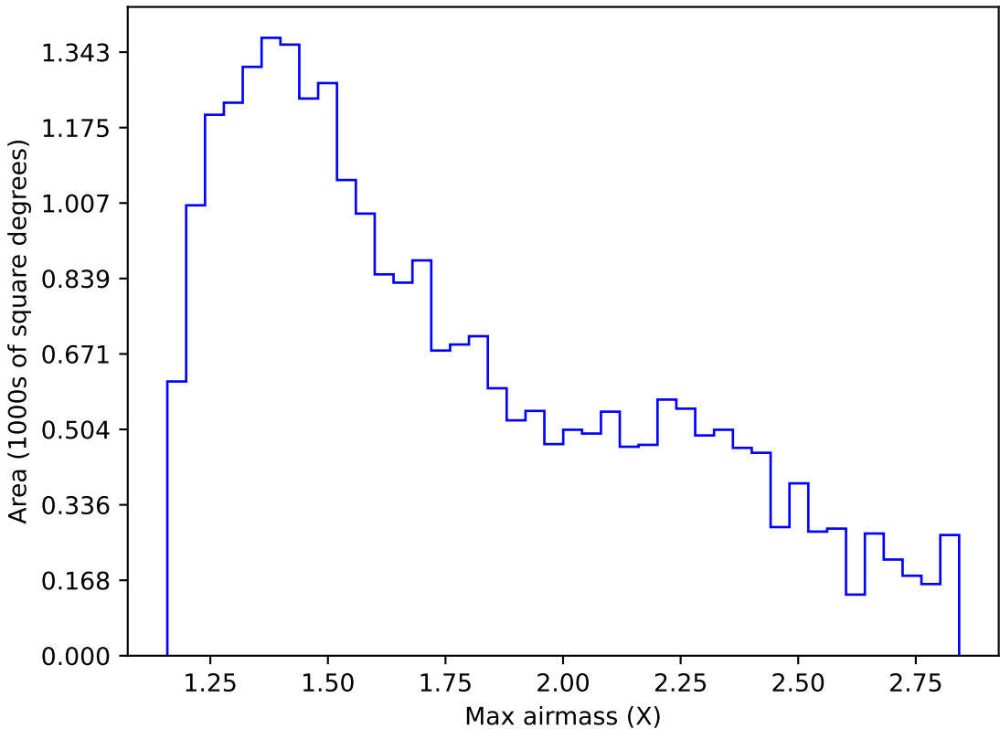
ddf_acor_sf10_lsf20_lsr10_v3.4_10yrs Yr 1 i band: Max airmass
