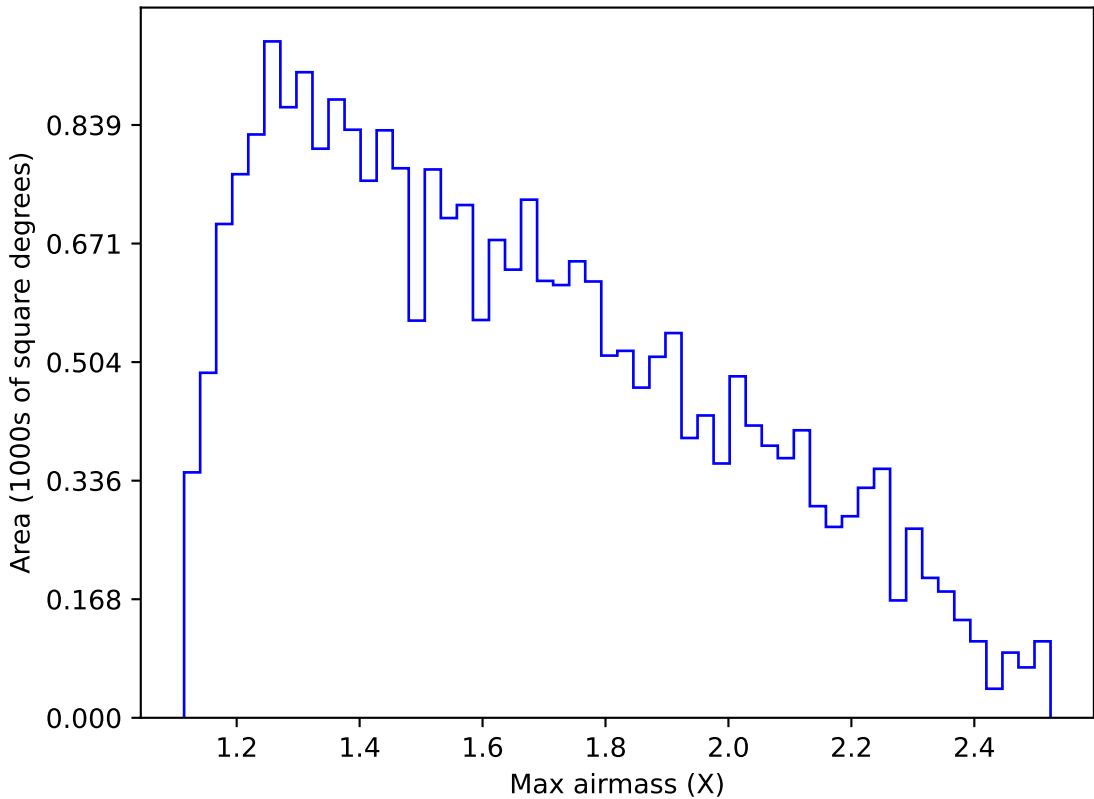
ddf_acor_sf10_lsf20_lsr10_v3.4_10yrs Yr 1 g band: Max airmass
