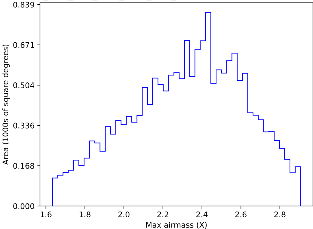
ddf_acor_sf10_ls20_lsr10_v3.4_10yrs WFD y band: Max airmass
