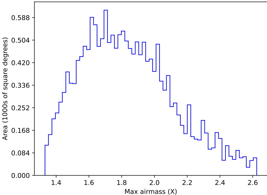
ddf_acor_sf10_lsf20_lsr10_v3.4_10yrs WFD u band: Max airmass
