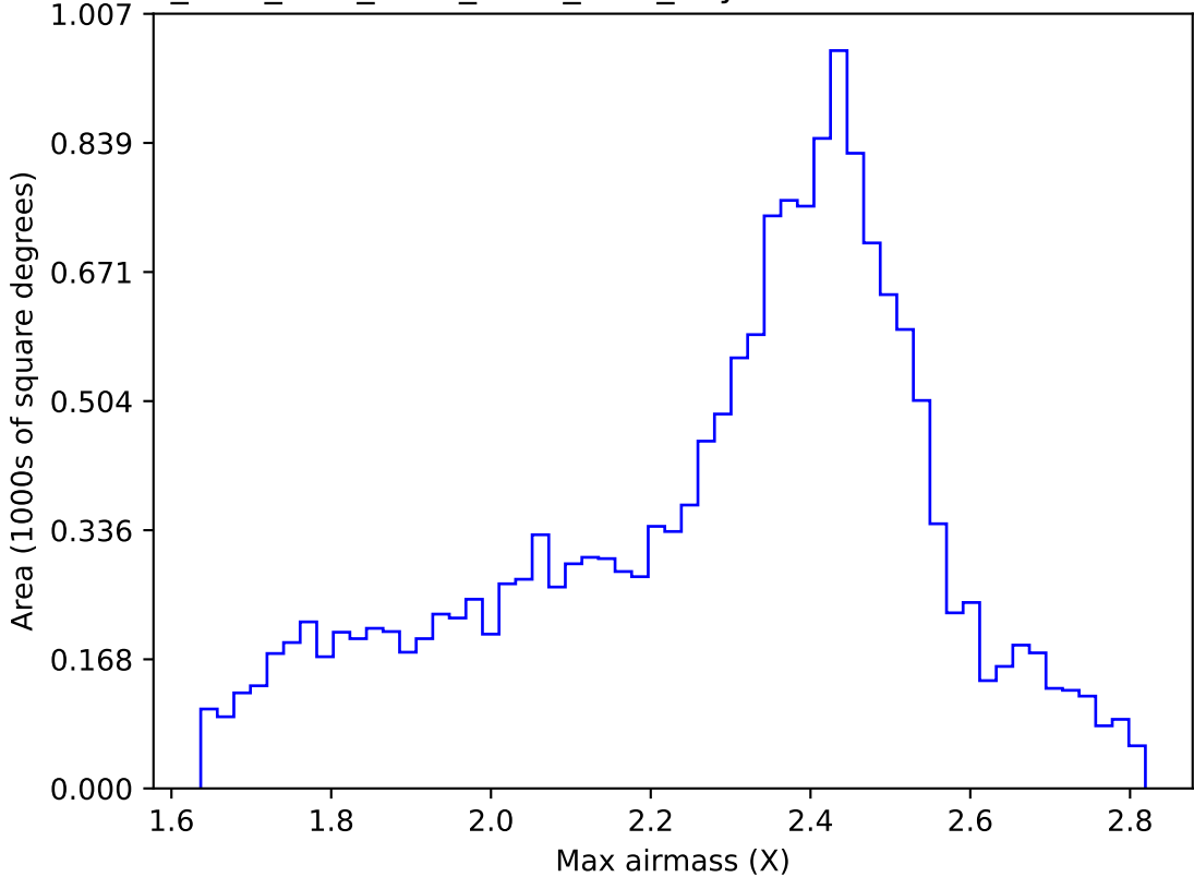
ddf_acor_sf10_lsf20_lsr10_v3.4_10yrs WFD r band: Max airmass
