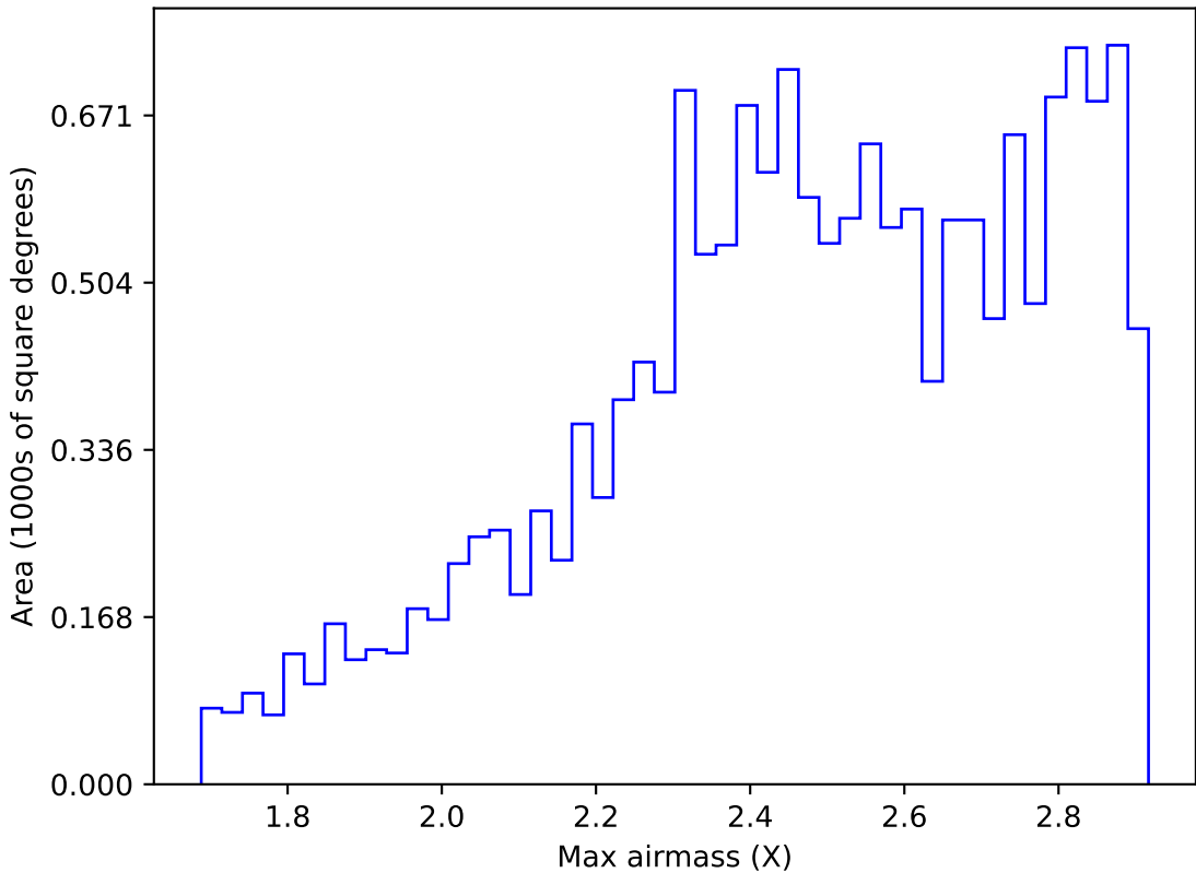
ddf_acor_sf10_lsf20_lsr10_v3.4_10yrs WFD i band: Max airmass
