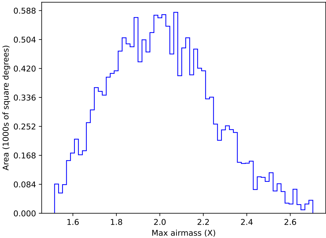
ddf_acor_sf10_lsf20_lsr10_v3.4_10yrs WFD g band: Max airmass
