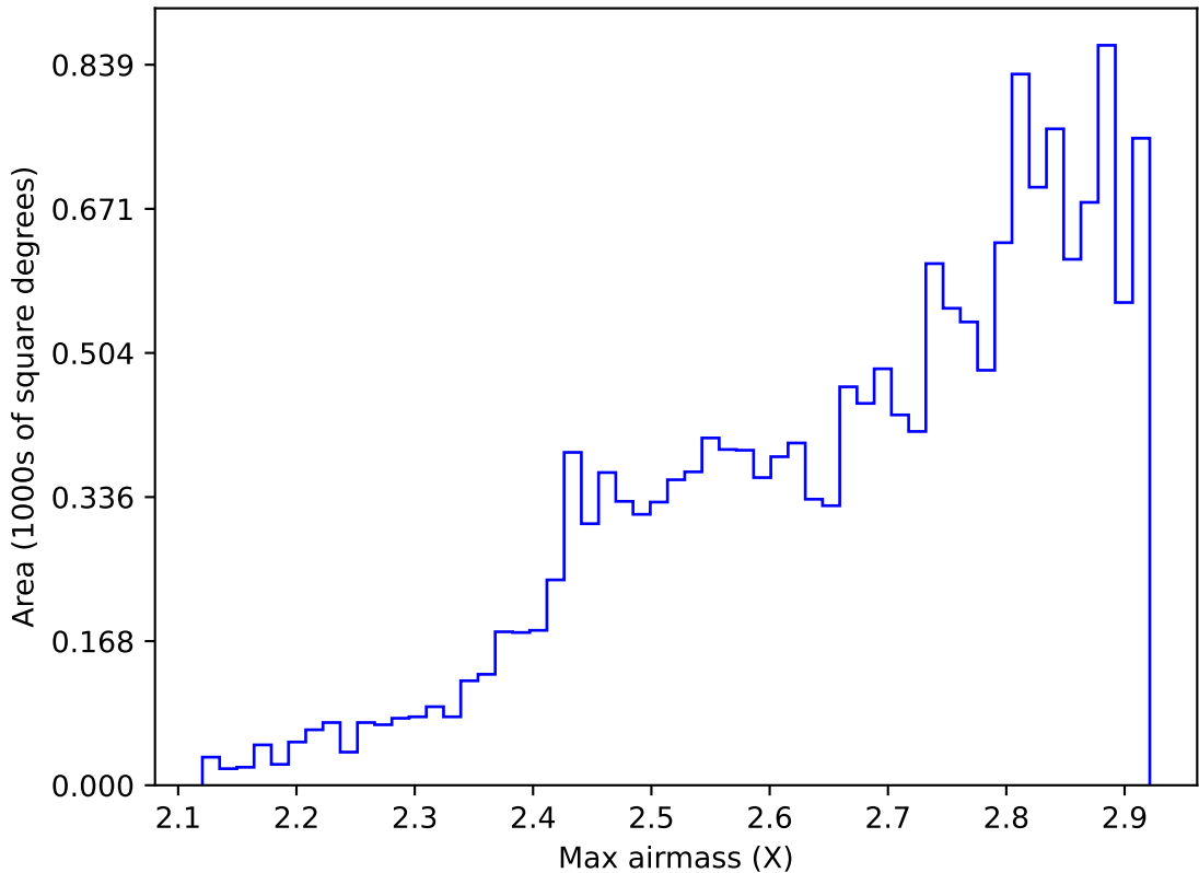
ddf_acor_sf10_lsf20_lsr10_v3.4_10yrs WFD all bands: Max airmass
