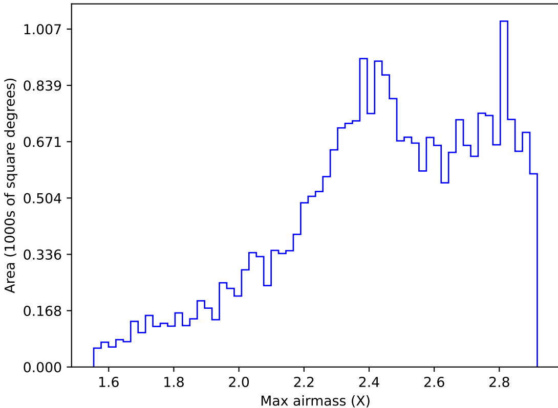
ddf_acor_sf10_lsf20_lsr10_v3.4_10yrs All sky z band: Max airmass
