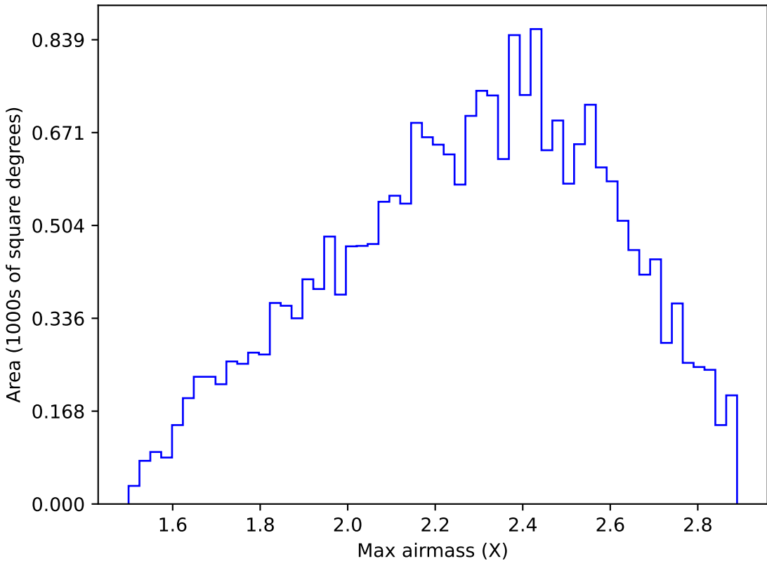
ddf_acor_sf10_lsf20_lsr10_v3.4_10yrs All sky y band: Max airmass
