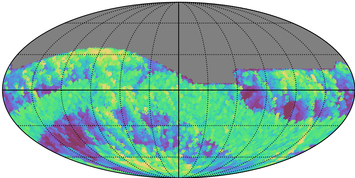
ddf_acor_sf10_lsf20_lsr10_v3.4_10yrs All sky r band: Max airmass
