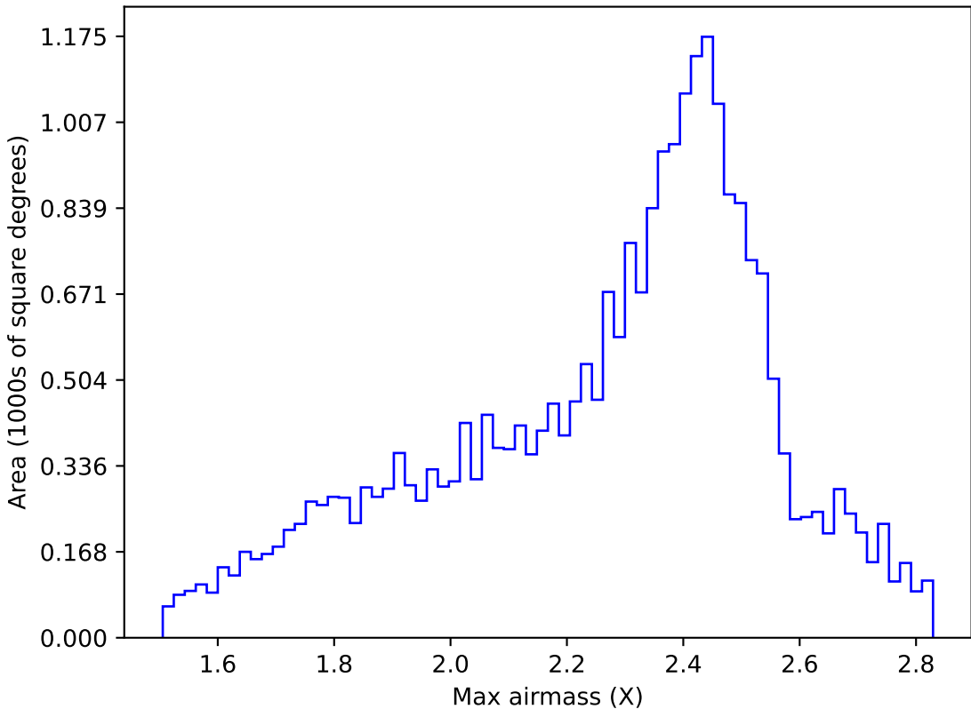
ddf_acor_sf10_lsf20_lsr10_v3.4_10yrs All sky r band: Max airmass
