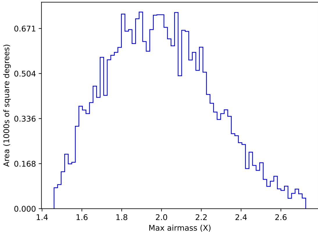
ddf_acor_sf10_lsf20_lsr10_v3.4_10yrs All sky g band: Max airmass
