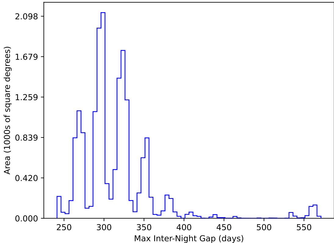
ddf_acor_sf10_lsf20_lsr10_v3.4_10yrs WFD y band: Max Inter-Night Gap
