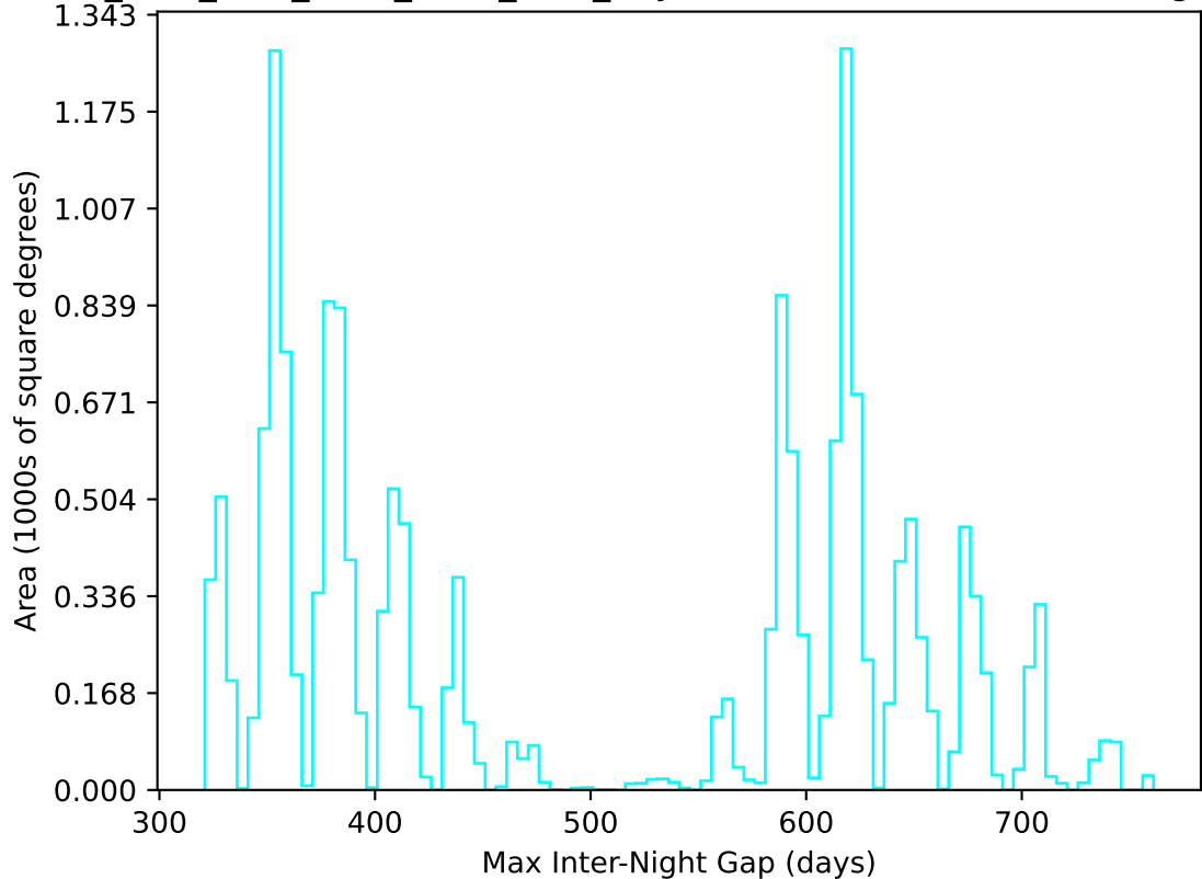
ddf_acor_sf10_lsf20_lsr10_v3.4_10yrs WFD u band: Max Inter-Night Gap
