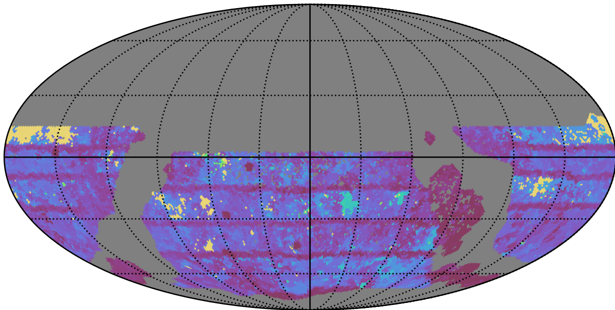
ddf_acor_sf10_lsf20_lsr10_v3.4_10yrs WFD r band: Max Inter-Night Gap
