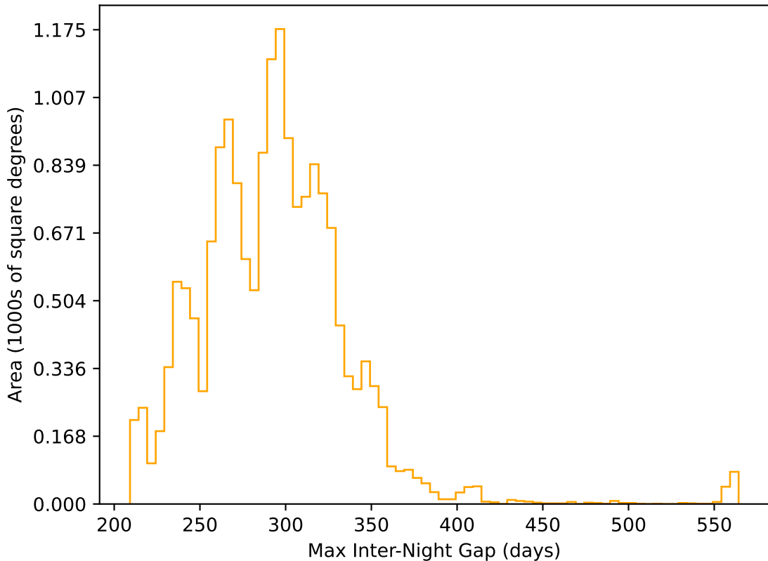
ddf_acor_sf10_lsf20_lsr10_v3.4_10yrs WFD r band: Max Inter-Night Gap
