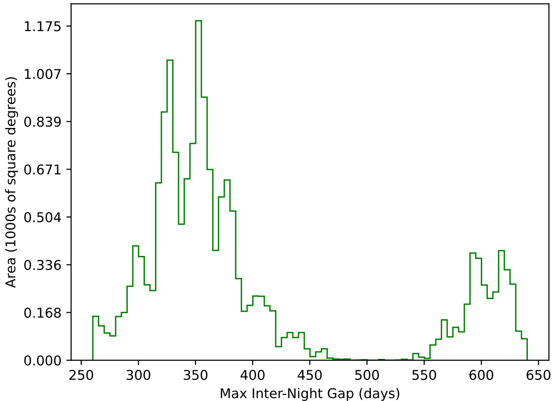
ddf_acor_sf10_lsf20_lsr10_v3.4_10yrs WFD g band: Max Inter-Night Gap
