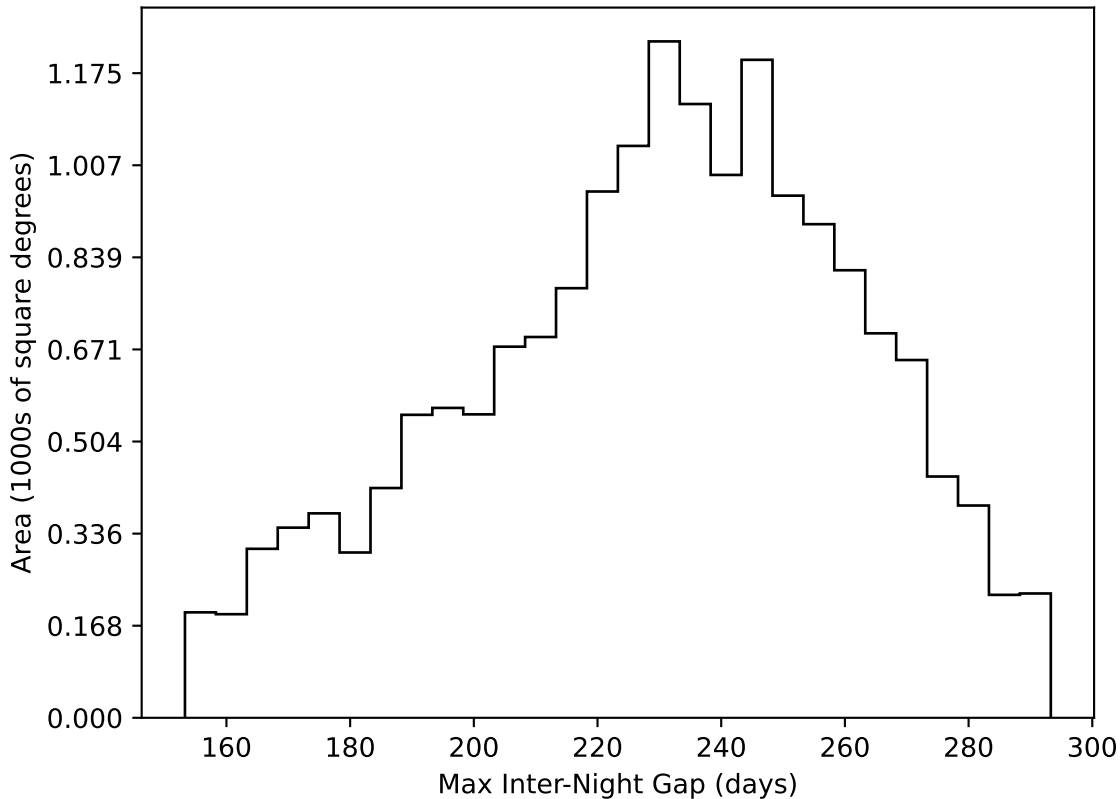
ddf_acor_sf10_lsf20_lsr10_v3.4_10yrs WFD all bands: Max Inter-Night Gap
