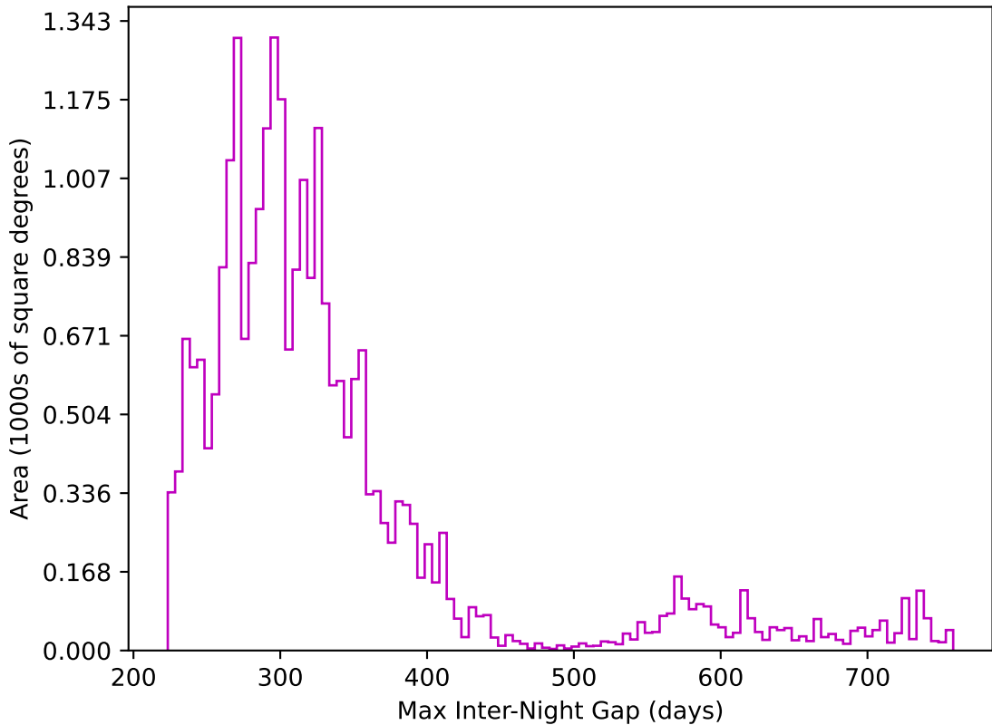
ddf_acor_sf10_lsf20_lsr10_v3.4_10yrs All sky z band: Max Inter-Night Gap
