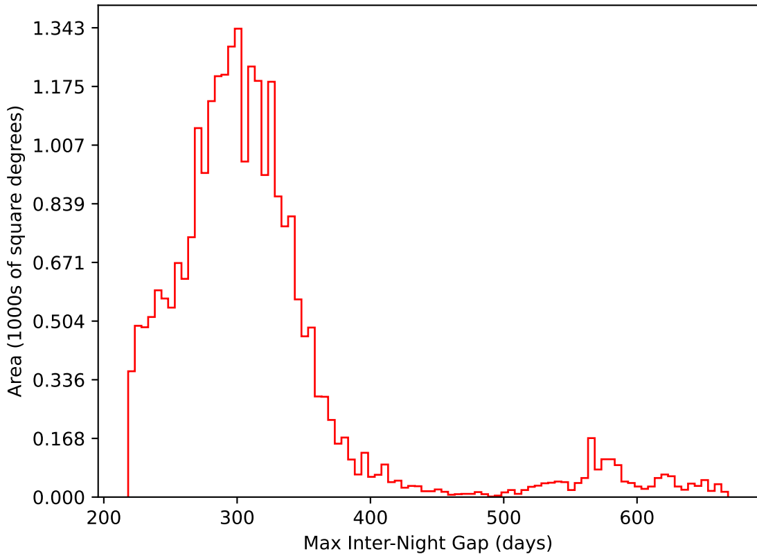
ddf_acor_sf10_lsf20_lsr10_v3.4_10yrs All sky i band: Max Inter-Night Gap
