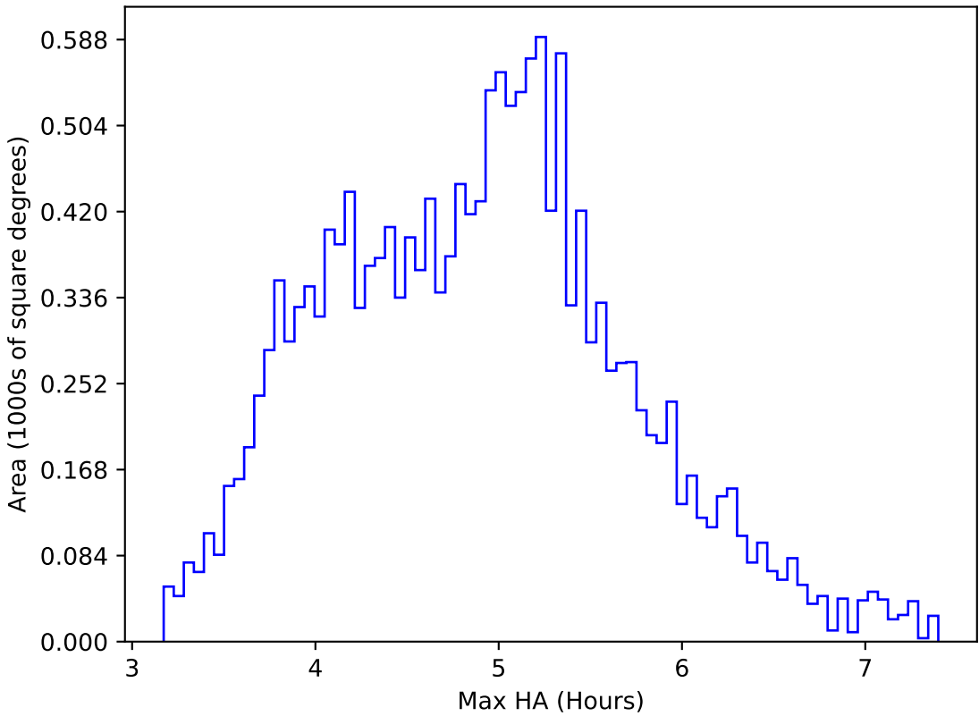
ddf_acor_sf10_lsf20_lsr10_v3.4_10yrs WFD z band: Max HA
