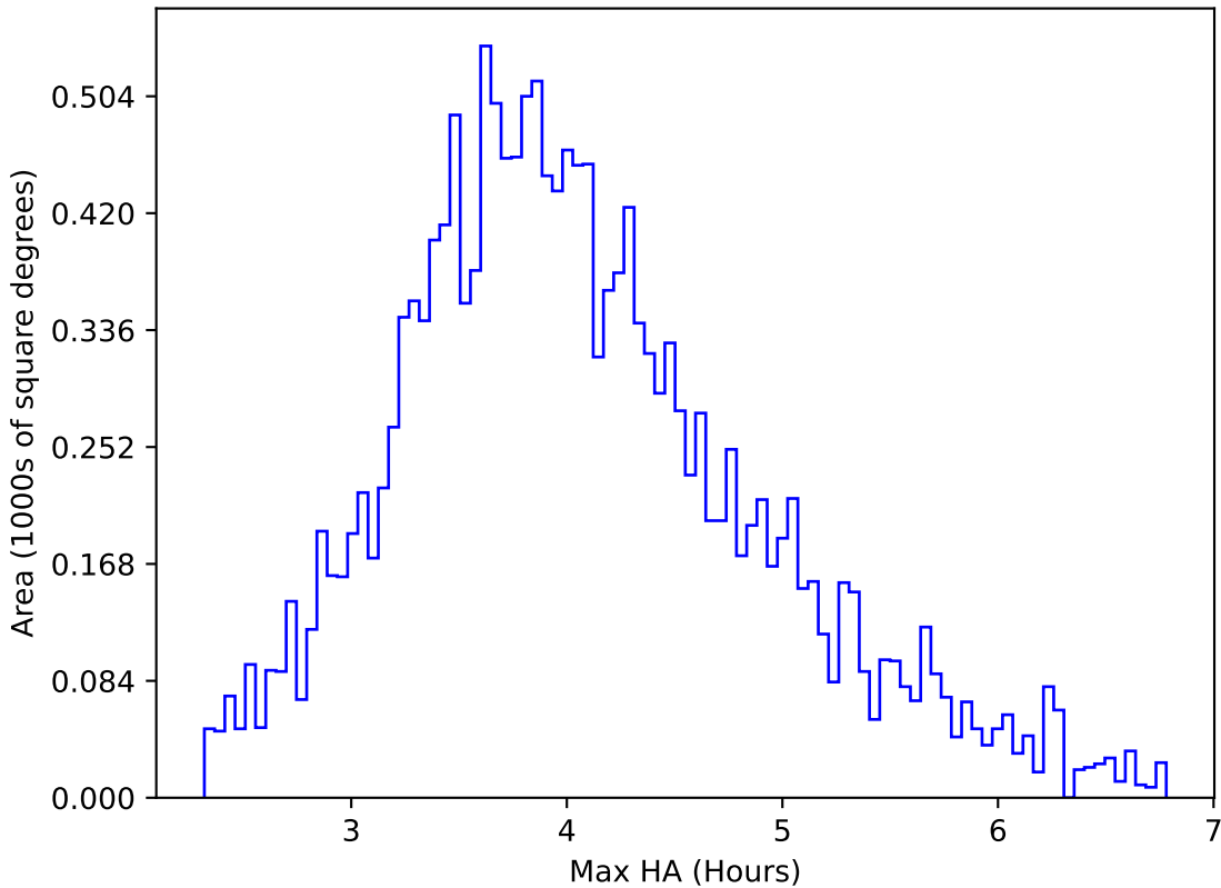
ddf_acor_sf10_lsf20_lsr10_v3.4_10yrs WFD g band: Max HA
