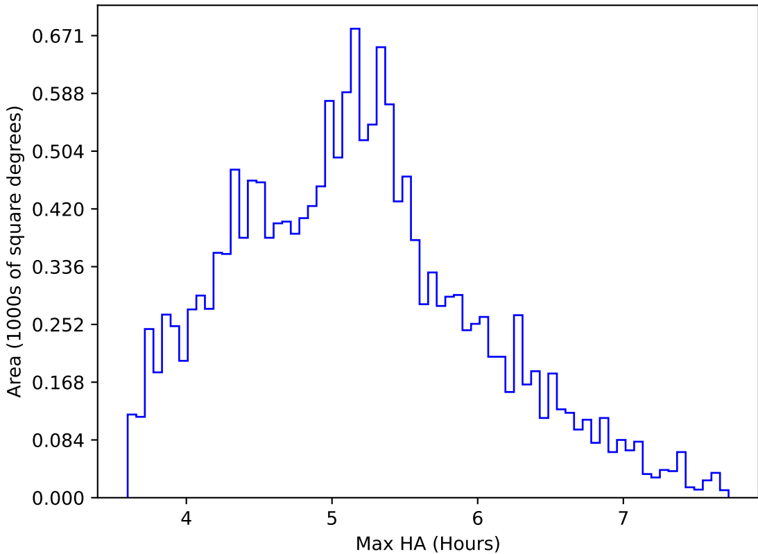
ddf_acor_sf10_lsf20_lsr10_v3.4_10yrs WFD all bands: Max HA
