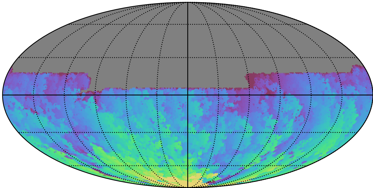
ddf_acor_sf10_lsf20_lsr10_v3.4_10yrs All sky u band: Max HA
