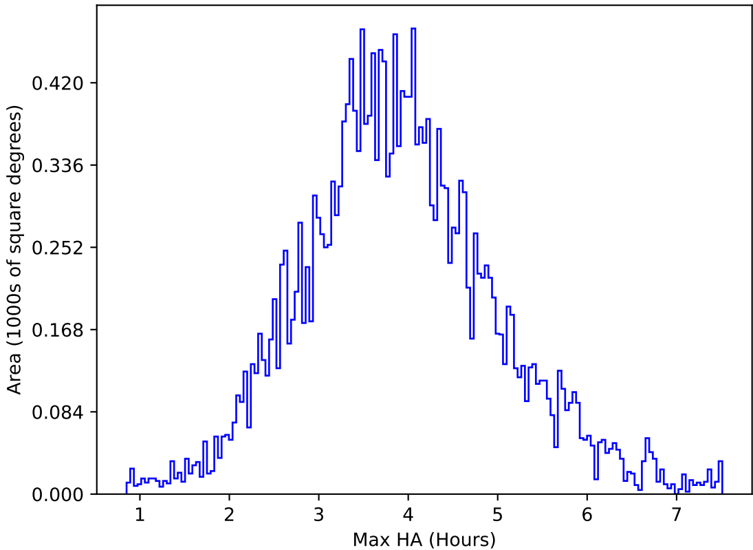
ddf_acor_sf10_lsf20_lsr10_v3.4_10yrs All sky u band: Max HA
