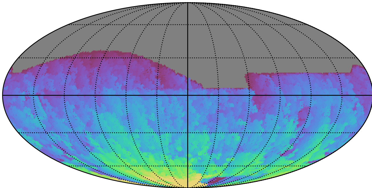
ddf_acor_sf10_lsf20_lsr10_v3.4_10yrs All sky r band: Max HA
