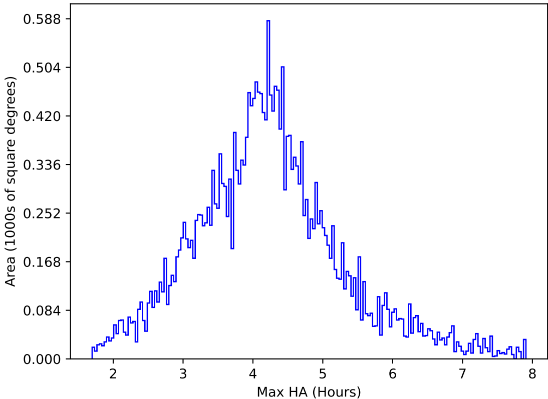
ddf_acor_sf10_ls20_lsr10_v3.4_10yrs All sky r band: Max HA
