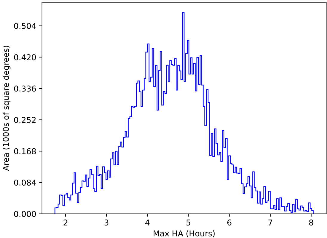
ddf_acor_sf10_lsf20_lsr10_v3.4_10yrs All sky i band: Max HA
