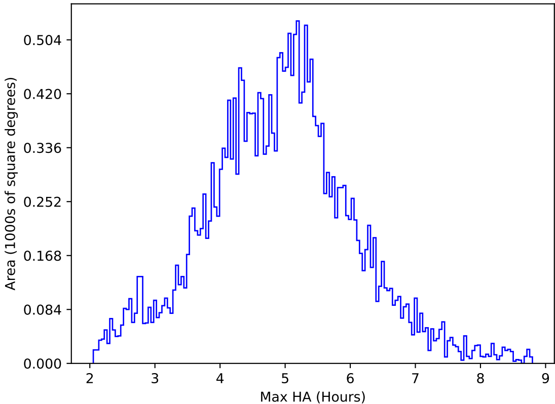
ddf_acor_sf10_lsf20_lsr10_v3.4_10yrs All sky all bands: Max HA
