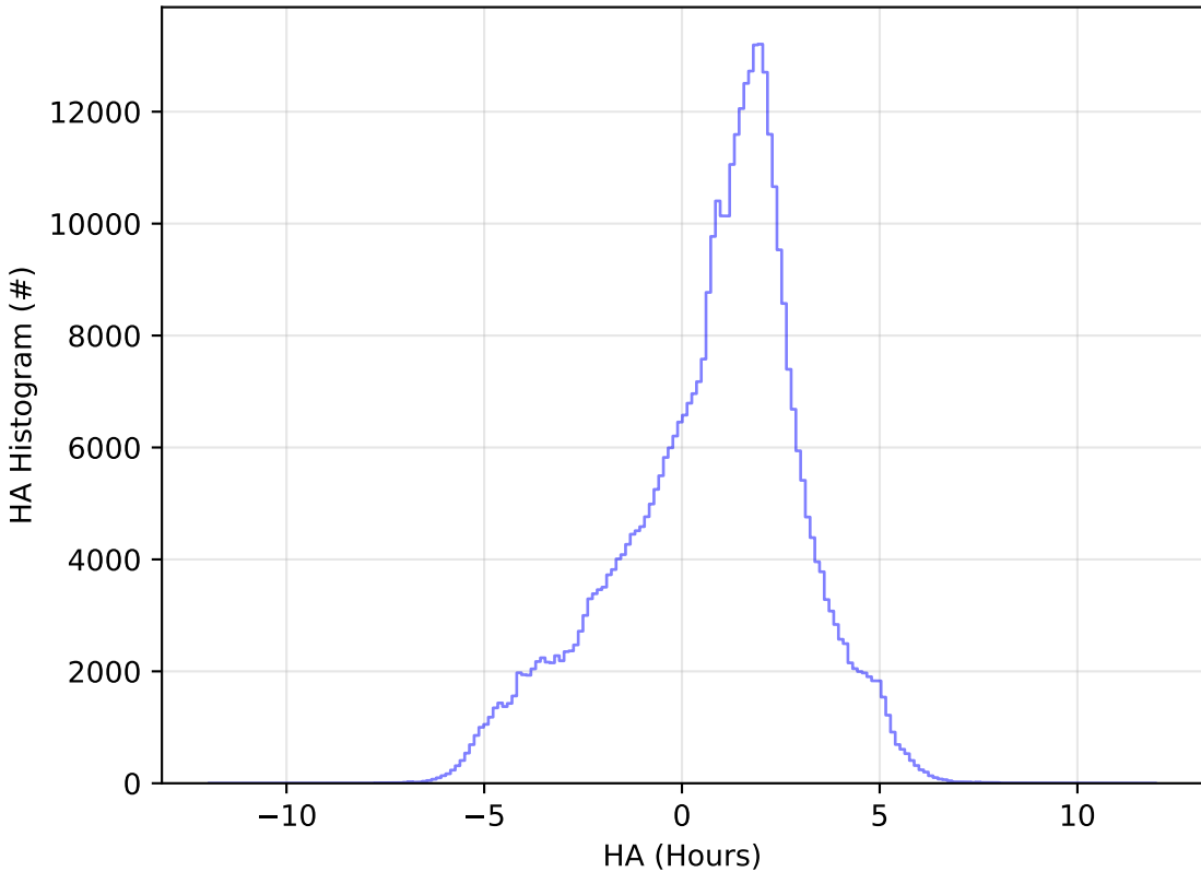
ddf_acor_sf10_lsf20_lsr10_v3.4_10yrs WFD z band: HA Histogram
