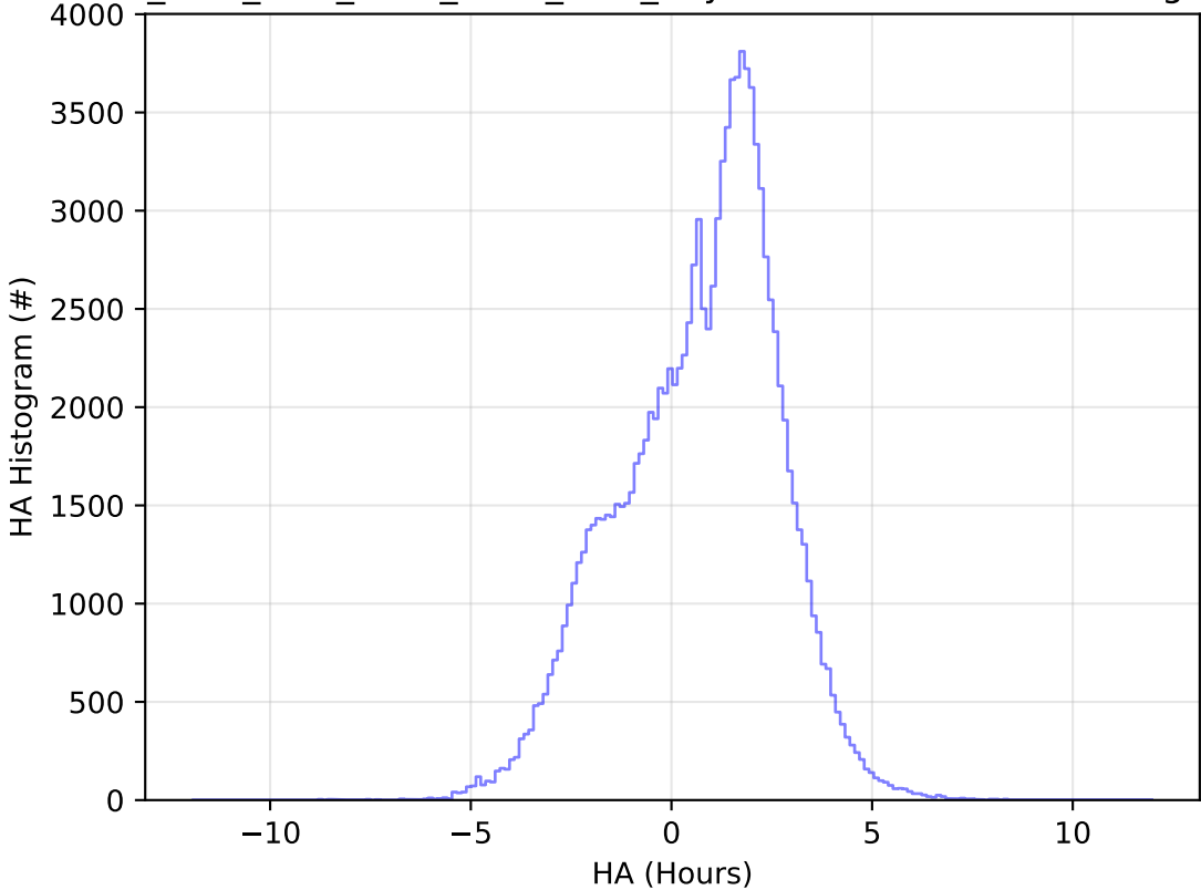
ddf_acor_sf10_lsf20_lsr10_v3.4_10yrs WFD u band: HA Histogram
