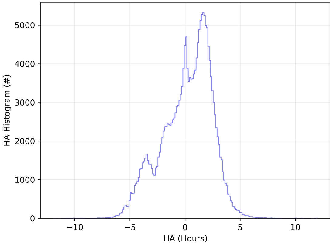
ddf_acor_sf10_lsf20_lsr10_v3.4_10yrs WFD g band: HA Histogram
