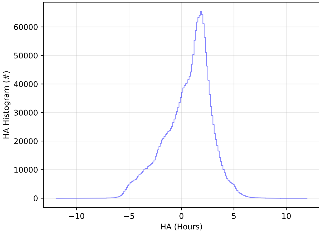
ddf_acor_sf10_lsf20_lsr10_v3.4_10yrs WFD all bands: HA Histogram
