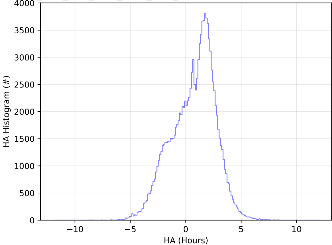
ddf_acor_sf10_lsf20_lsr10_v3.4_10yrs All sky u band: HA Histogram
