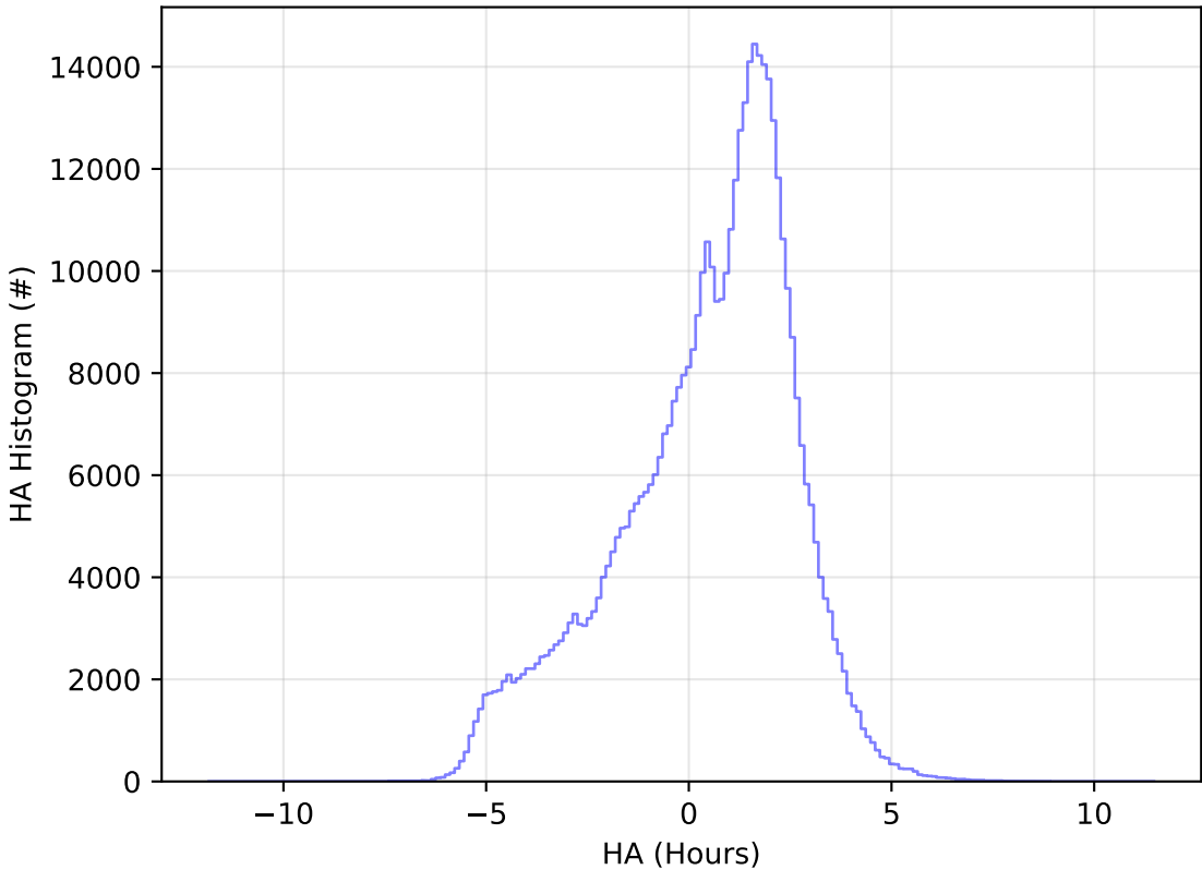
ddf_acor_sf10_lsf20_lsr10_v3.4_10yrs All sky r band: HA Histogram
