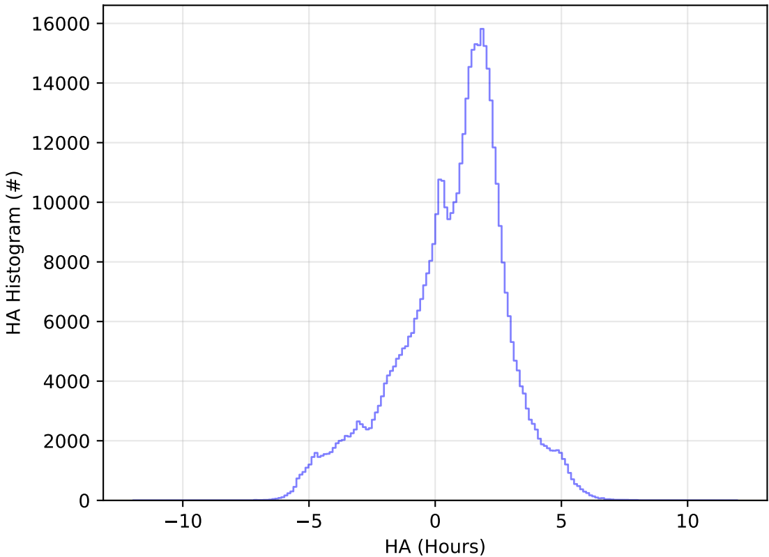
ddf_acor_sf10_lsf20_lsr10_v3.4_10yrs All sky i band: HA Histogram
