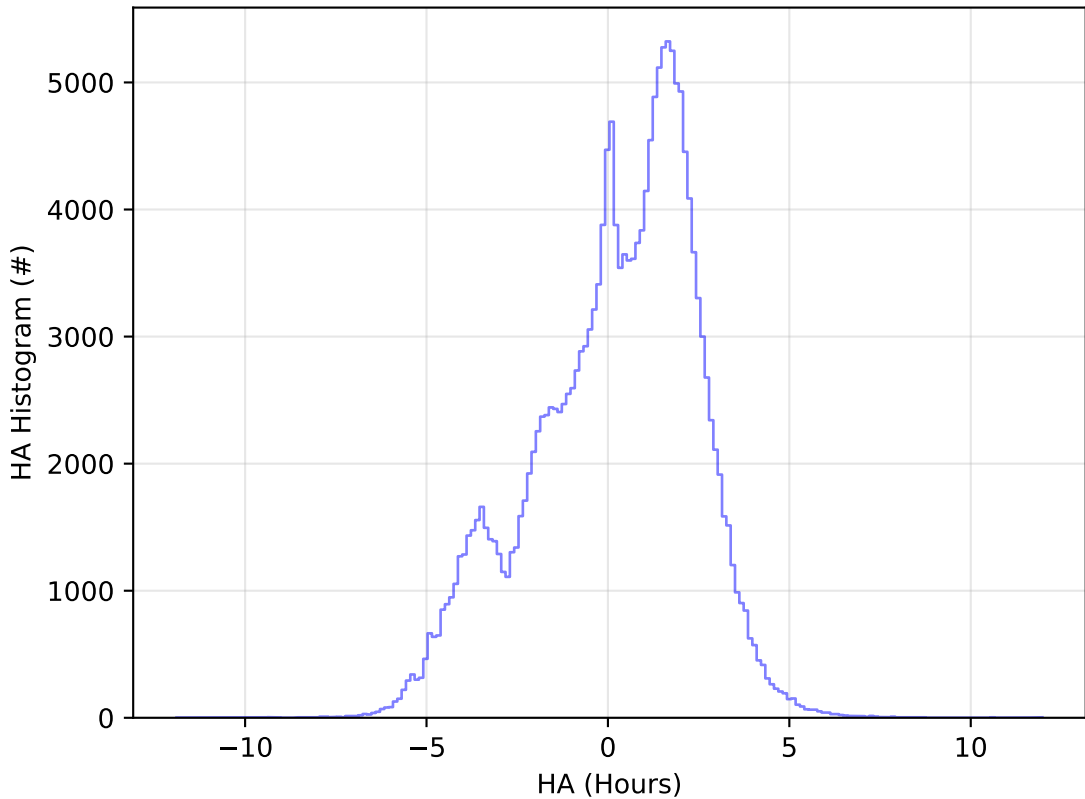
ddf_acor_sf10_lsf20_lsr10_v3.4_10yrs All sky g band: HA Histogram
