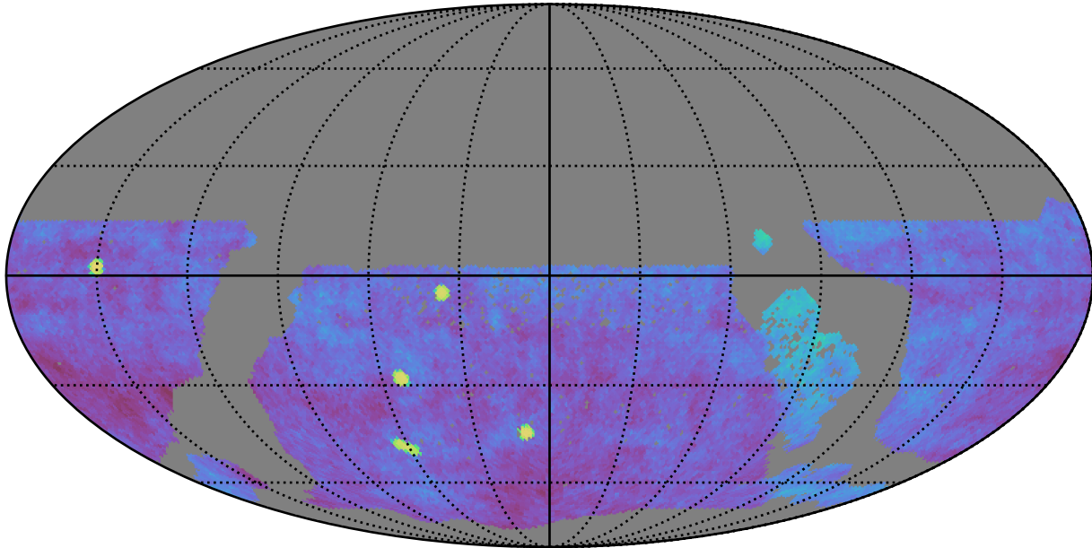
ddf_acor_sf10_lsf20_lsr10_v3.4_10yrs gri WFD: Fraction of visits in pairs (10-60 min)
