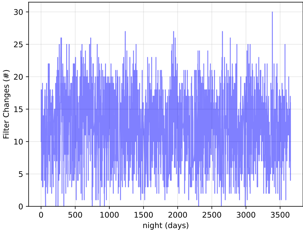
ddf_acor_sf10_lsf20_lsr10_v3.4_10yrs Per Night: Filter Changes
