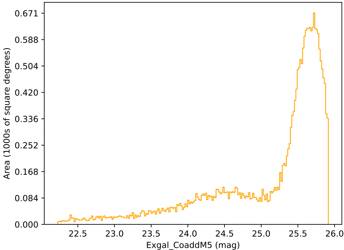
ddf_acor_sf10_lsf20_lsr10_v3.4_10yrs Yr 1 r band: Exgal_CoaddM5
